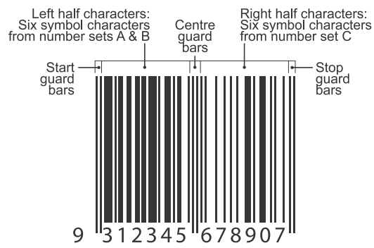
Figure 2 - EAN-13 Bar Code Format
